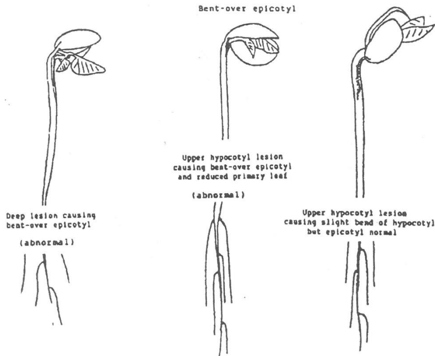
Fig. 3 Bent-over Epicotyl
