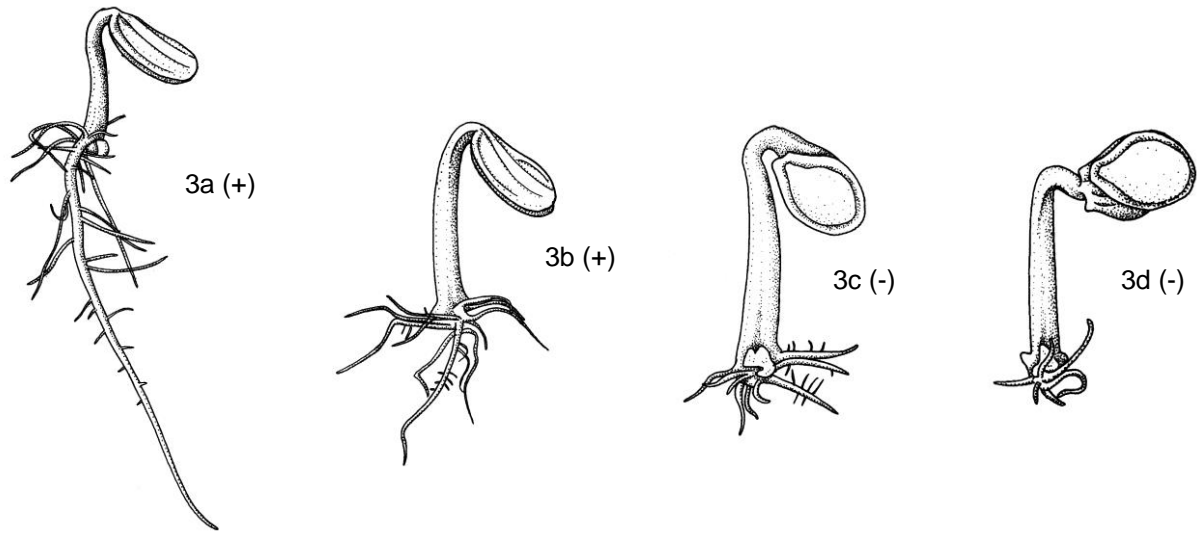
Fig. 3 Root defects.
