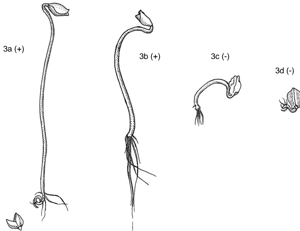
Fig. 3 Root defects.
