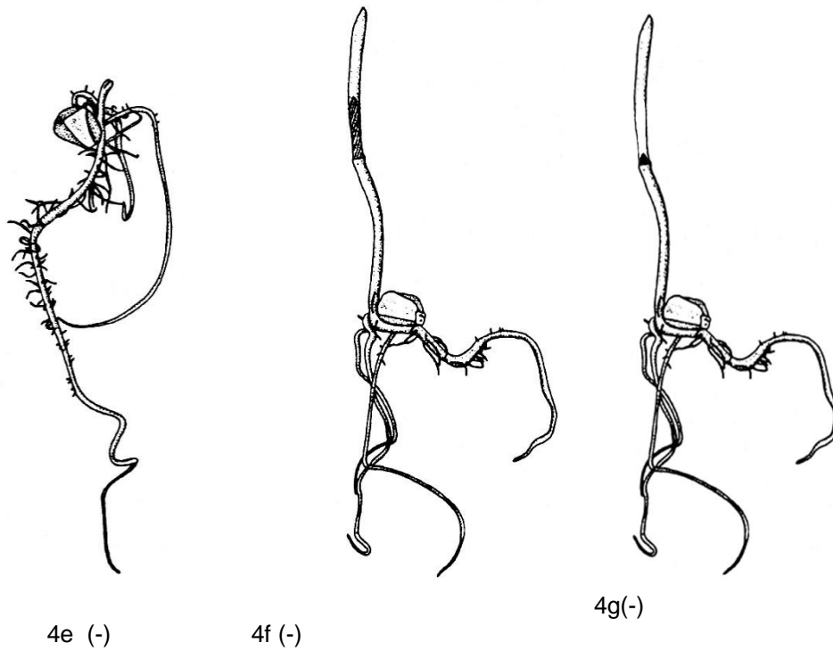
Fig. 5 Mesocotyl defects.
