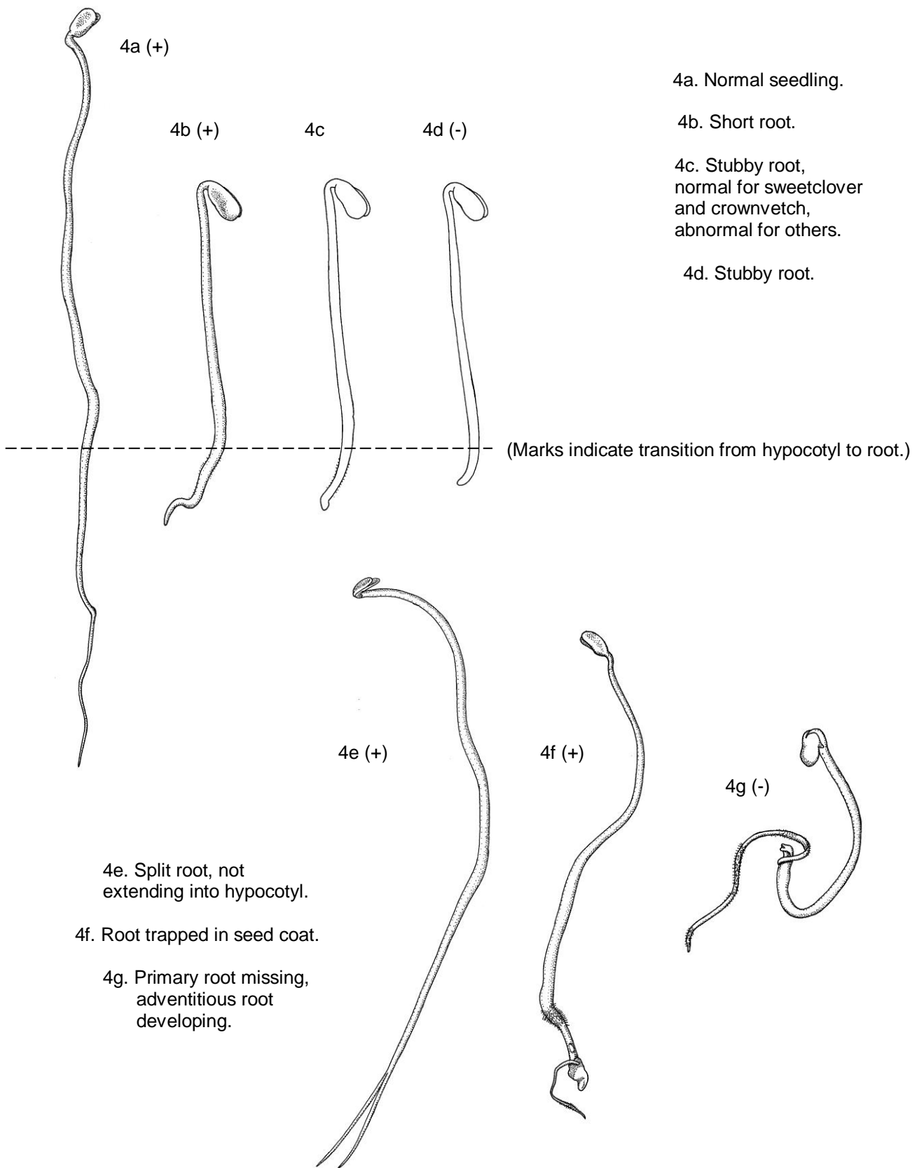
Fig. 4 Root Defects
