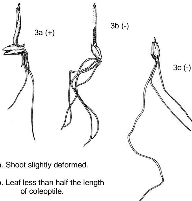
Fig. 3 Shoot defects.
