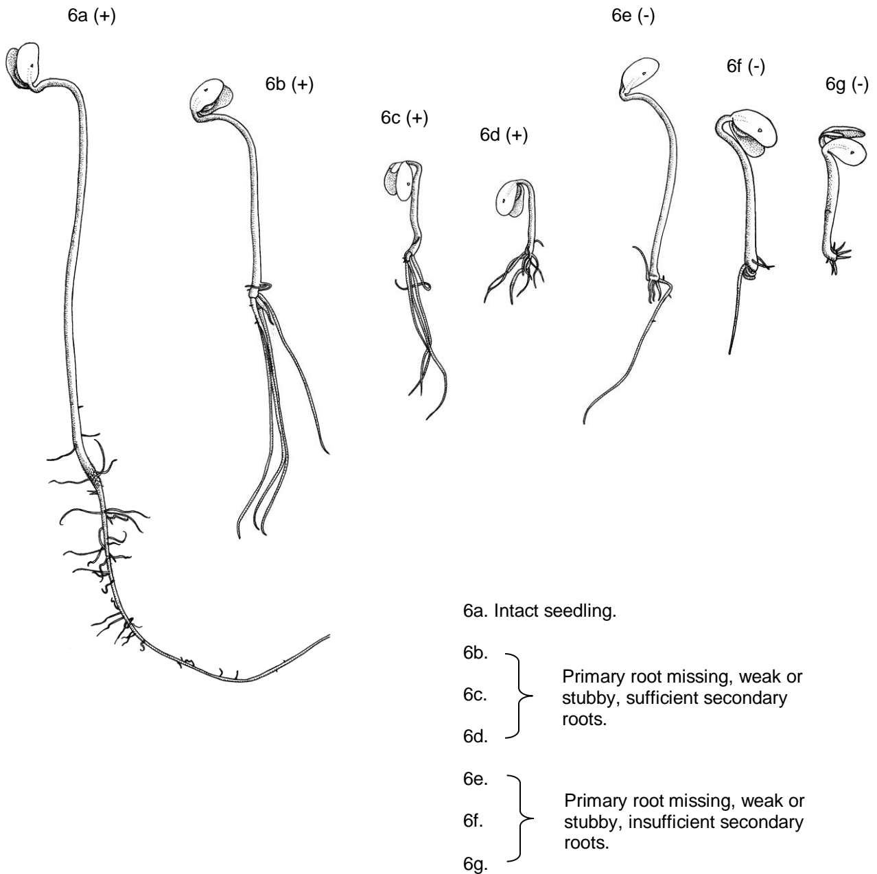
Fig. 6 Root defects.
