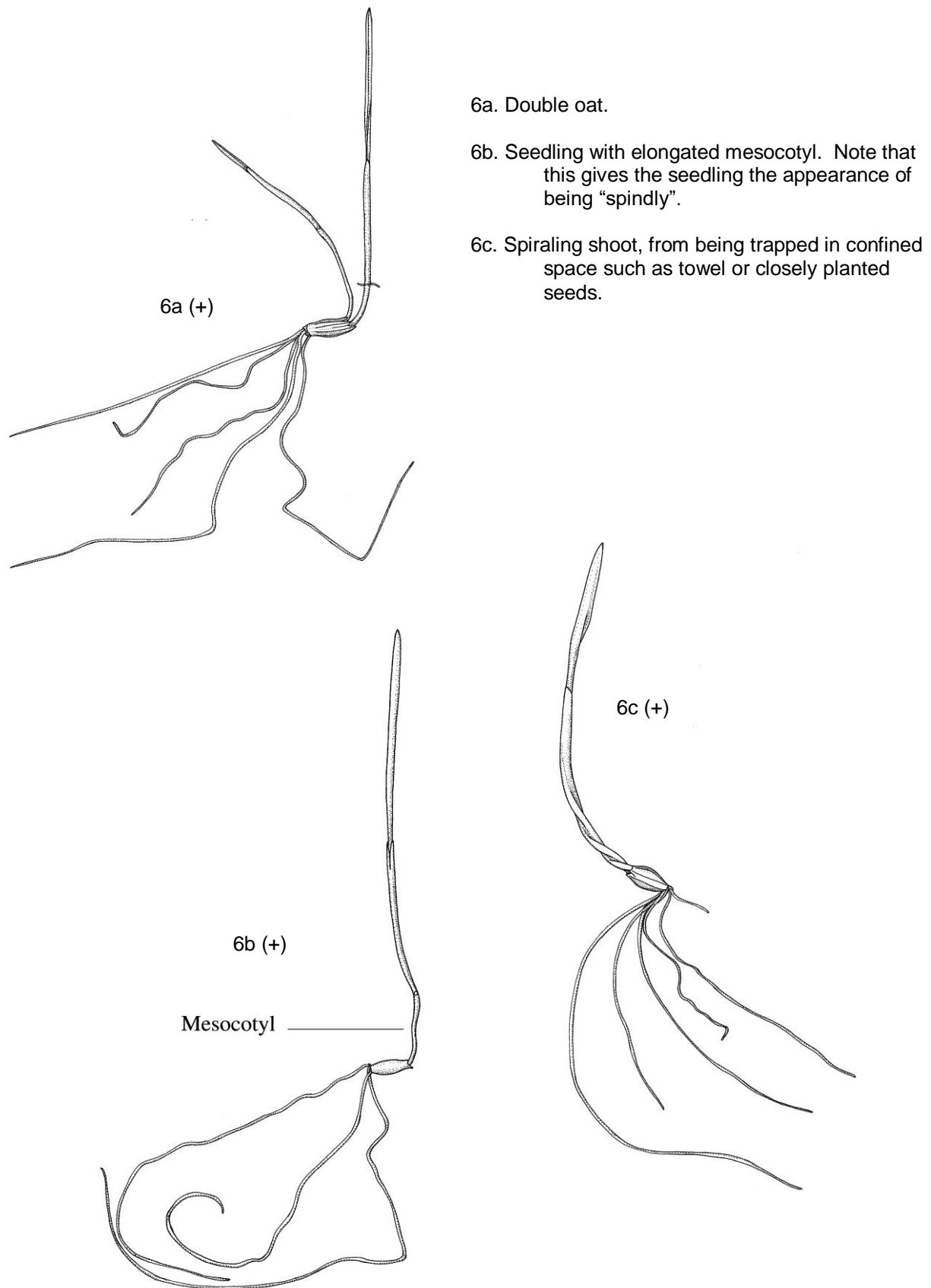
Fig. 6 Seedlings.
