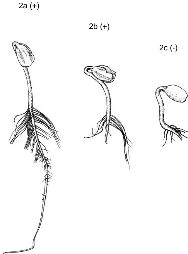
Fig. 4 Small seedlings.
