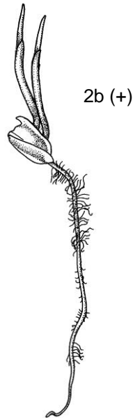
Fig. 2 Shoot defects.
